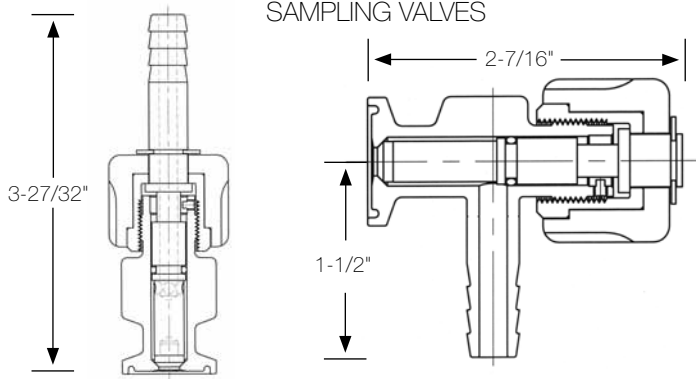
SAMPLING VALVES
